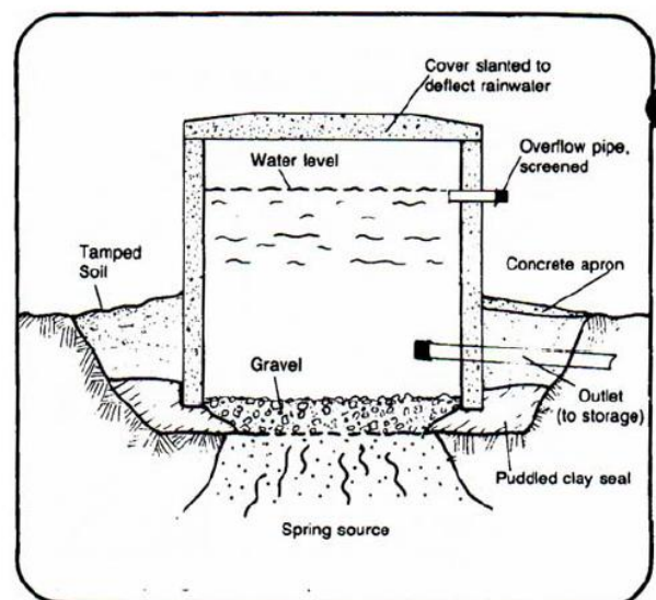
Figure 3: Spring box with permeable bottom that will be the model for the improved spring in Parina. (Courtesy of USAID, 1982, available online at www.lifewater.org )
